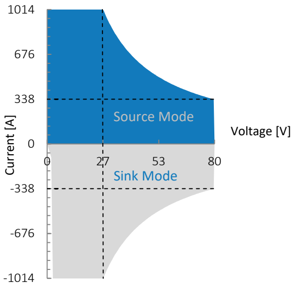
Figure 1: G5.RSS.27.80.1014, voltage / current operating area.
