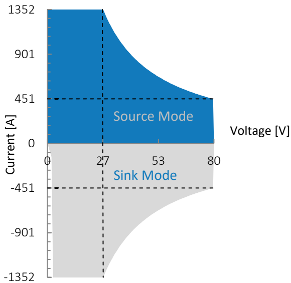
Figure 1: G5.RSS.36.80.1352, voltage / current operating area.
