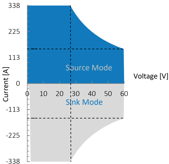
Figure 1: G5.RSS.9.60.338, voltage / current operating area.
