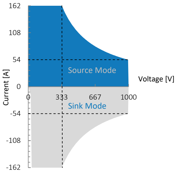
Figure 1: G5.RSS.54.1000.162, voltage / current operating area.
