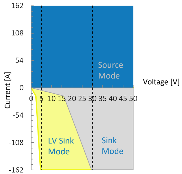
Figure 2: Normal sink mode in grey area down to 15(30) V. To use the LV Sink mode (yellow area), the upper voltage limit has to be lowered, - to 20 V for sink down to 2(5) V (yellow area) - to 332 V or higher for sink down to 15(30) V (grey area) - any other value between 20 V and 332 V will lead to a minimum sink voltage between 2(5) V and 15(30) V.
