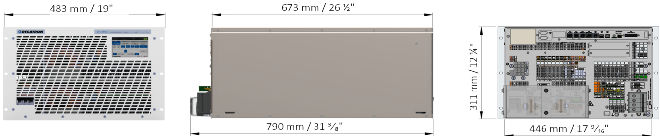
Figure 3: Front, right hand side and rear view. 19-inch module with 7 units in height. Add 130 mm / 5 1/8" to case depth for protective cover.
