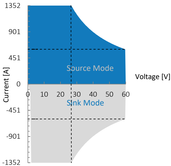
Figure 1: G5.RSS.36.60.1352, voltage / current operating area.
