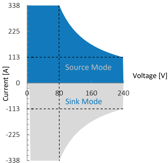
Figure 1: G5.RSS.27.240.338, voltage / current operating area.
