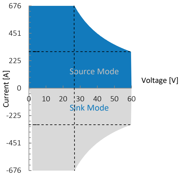
Figure 1: G5.RSS.18.60.676, voltage / current operating area.
