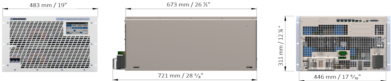
Figure 3: Front, right hand side and rear view. 19-inch module with 7 units in height. Add 74 mm / 2 7/8" to case depth for protective cover.
