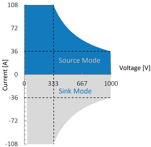
Figure 1: G5.RSS.36.1000.108, voltage / current operating area.
