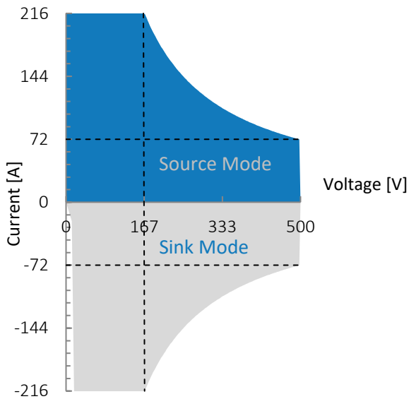
Figure 1: G5.RSS.36.500.216, voltage / current operating area.
