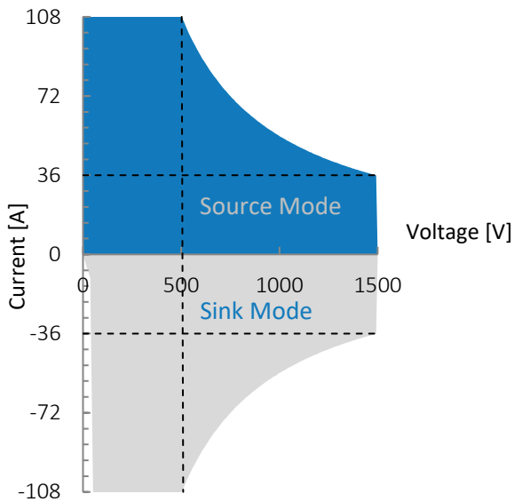
Figure 1: G5.RSS.54.1500.108, voltage / current operating area.
