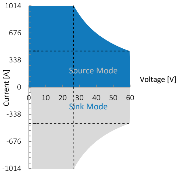
Figure 1: G5.RSS.27.60.1014, voltage / current operating area.
