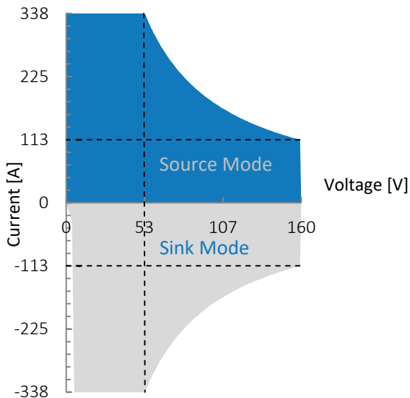
Figure 1: G5.RSS.18.160.338, voltage / current operating area.
