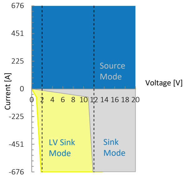
Figure 2: Normal sink mode in grey area down to 11(12) V. To use the LV Sink mode (yellow area), the upper voltage limit has to be lowered, - to 4 V for sink down to 1(2) V (yellow area) - to 52 V or higher for sink down to 11(12) V (grey area) - any other value between 4 V and 52 V will lead to a minimum sink voltage between 1(2) V and 11(12) V.
