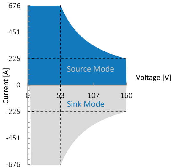
Figure 1: G5.RSS.36.160.676, voltage / current operating area.
