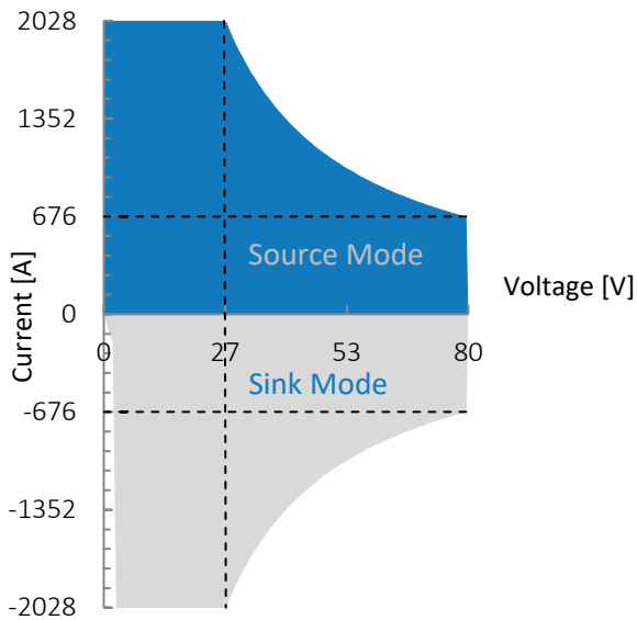
Figure 1: G5.RSS.54.80.2028, voltage / current operating area.
