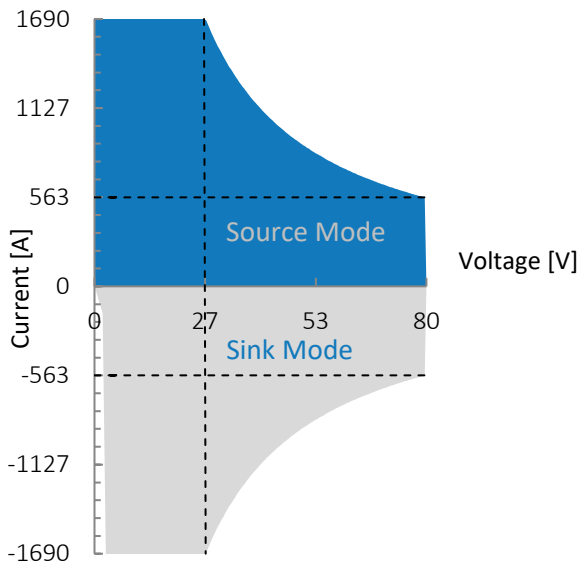
Figure 1: G5.RSS.45.80.1690, voltage / current operating area.
