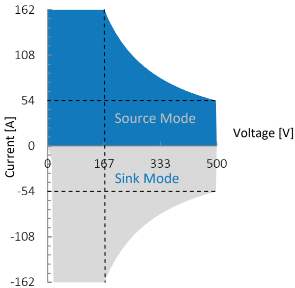
Figure 1: G5.RSS.27.500.162, voltage / current operating area.
