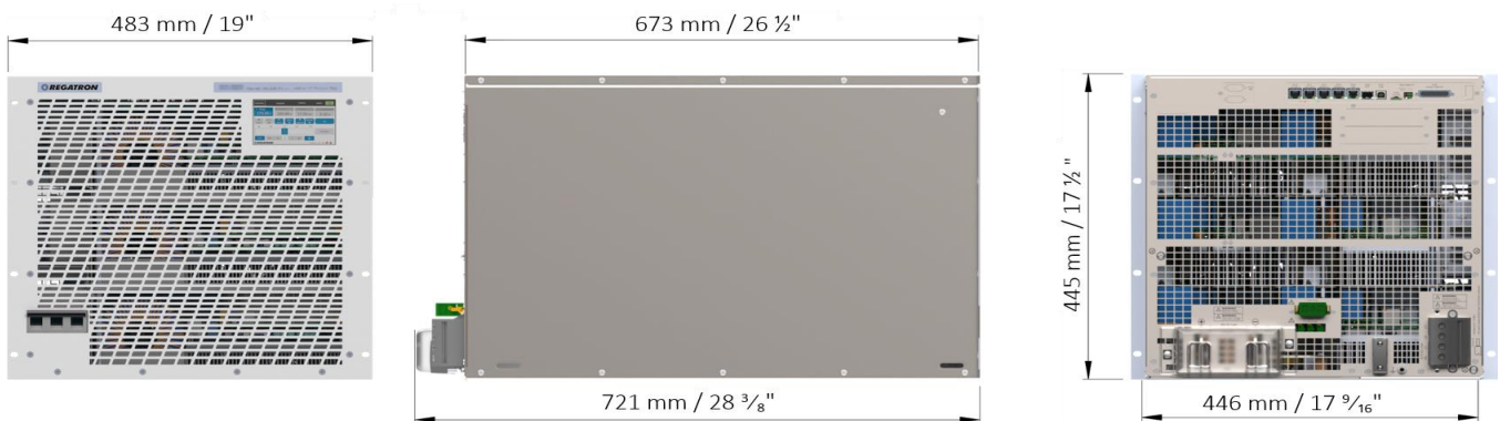
Figure 3: Front, right hand side and rear view. 19-inch module with 10 units in height. Add 74 mm / 2 7/8" to case depth for protective cover.
