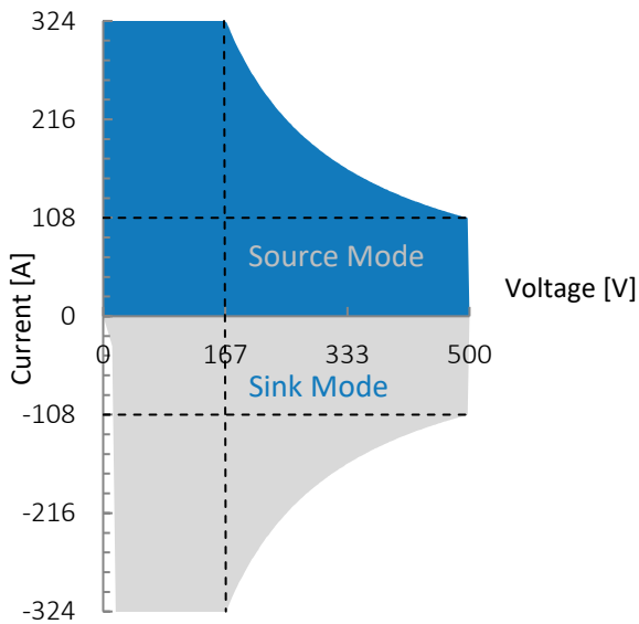
Figure 1: G5.RSS.54.500.324, voltage / current operating area.
