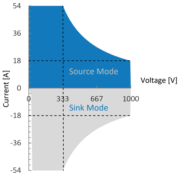
Figure 1: G5.RSS.18.1000.54, voltage / current operating area.
