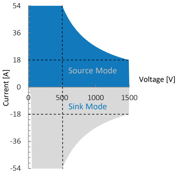
Figure 1: G5.RSS.27.1500.54, voltage / current operating area.
