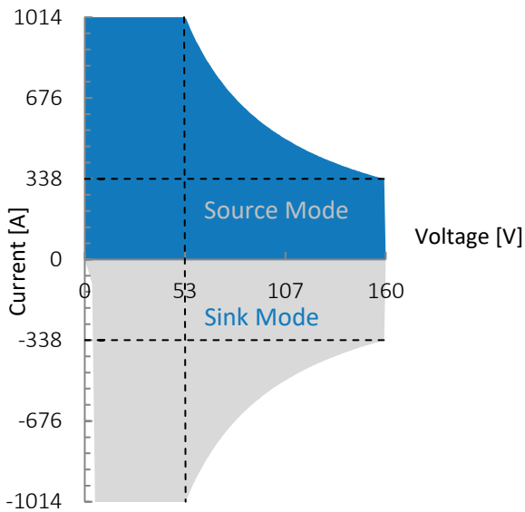
Figure 1: G5.RSS.54.160.1014, voltage / current operating area.
